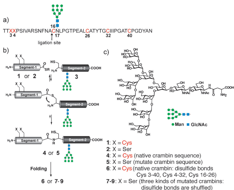
Figure 2. a) Amino-acid sequence of crambin: cysteines are highlighted in red and mutations are indicated by "X". b) General scheme for native chemical ligation (NCL) with the potential number of final products for the correctly folded 6 and mutated folded glycosyl crambins 7 , 8 , and 9 (three possible combinations for the four cysteines in the mutant 5 ). c) Tri-antennary high-mannose oligosaccharide.
