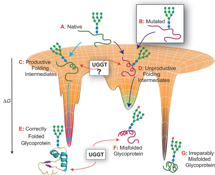
Figure 1. UGGT inspection during the glycoprotein folding process. Native glycoproteins A can follow a productive folding course to yield correctly folded glycoproteins (E), or an unproductive folding course, thus providing misfolded glycoprotein F, which can be re-glucosylated by UGGT for an additional folding attempt and can finally generate irreparably misfolded glycoproteins G, which will eventually be disposed of.
